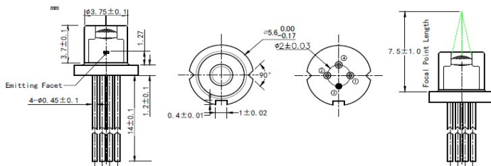
Product Package View: TO18 (5.6mm) Package:
